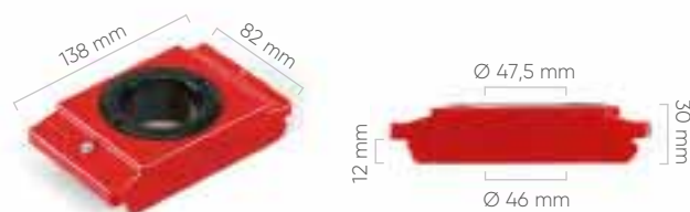
BOCCOLA HSK A63-B80
