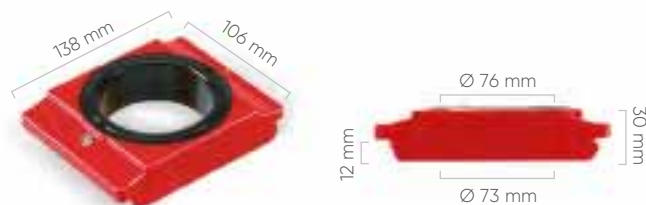
BOCCOLA HSK A100-B125
