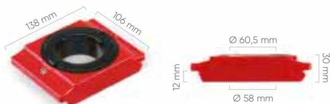
BOCCOLA HSK A80-B100
